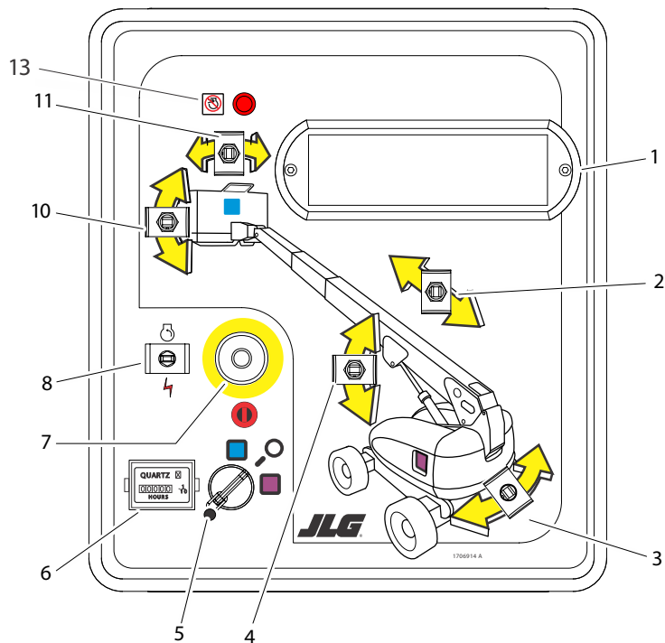
Figure 3-1. Console de commande au sol – 800S sans MSSO
