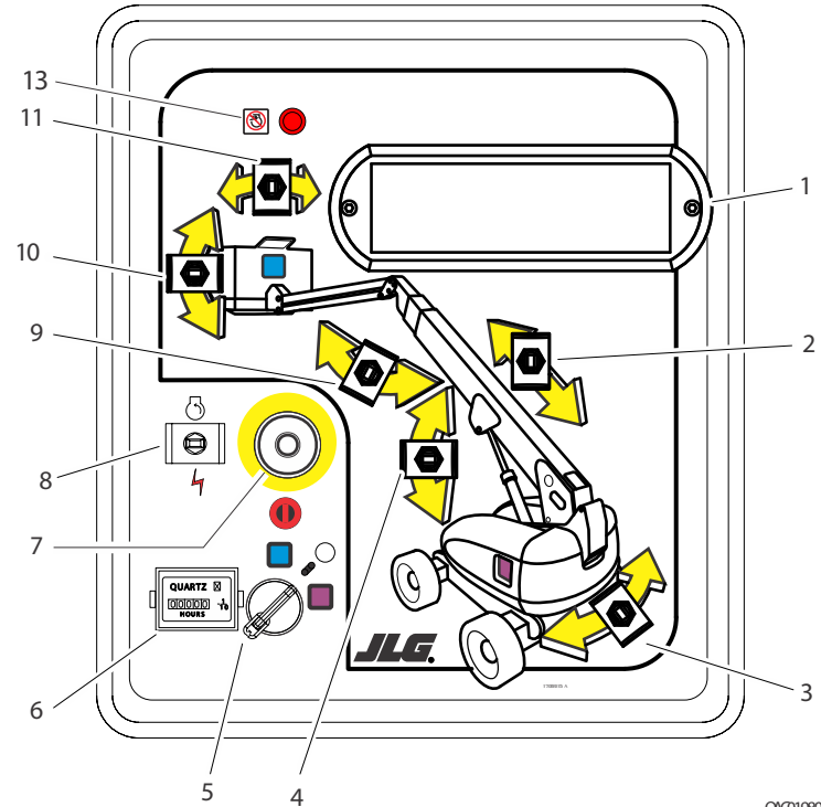
Figure 3-4. Console de commande au sol – 860SJ sans MSSO
